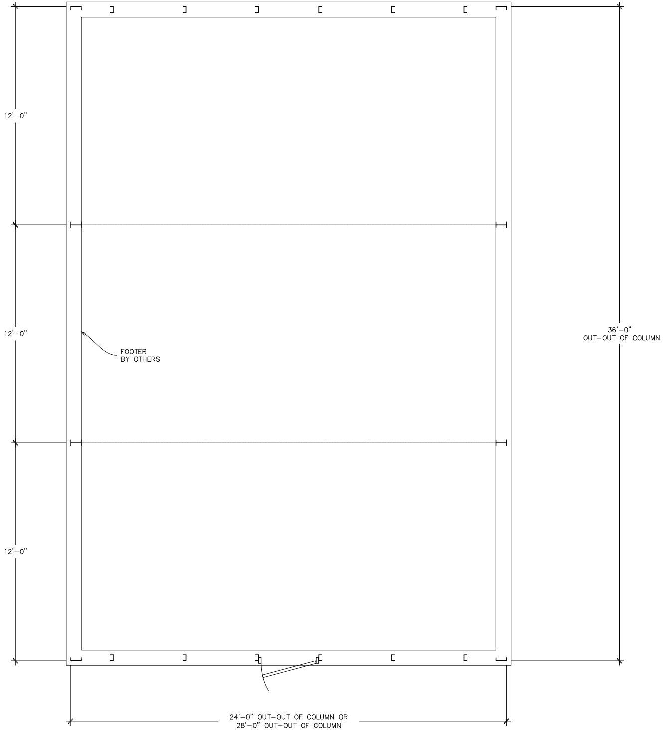
COLUMN LAYOUT
