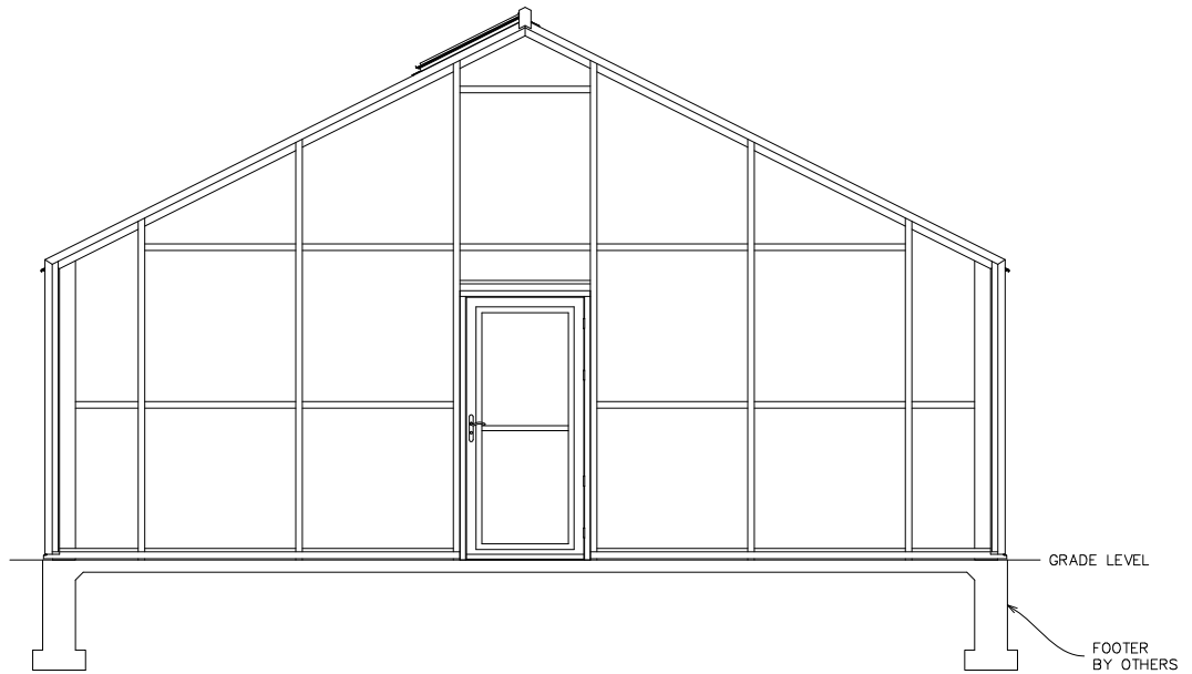
GABLE ELEVATION
